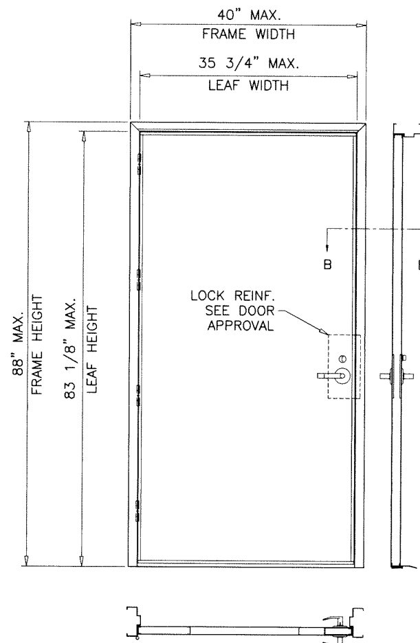
OUTSWING SINGLE STEEL DOOR
