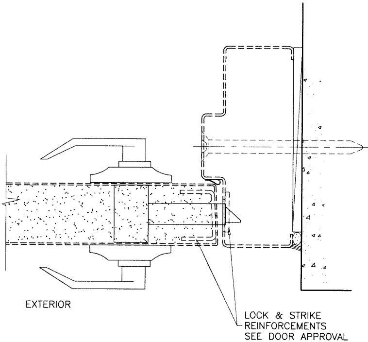
SECTION A-A 'GT' SERIES CYLINDRICAL LOCK 'XGT' SERIES LEVER LOCK
