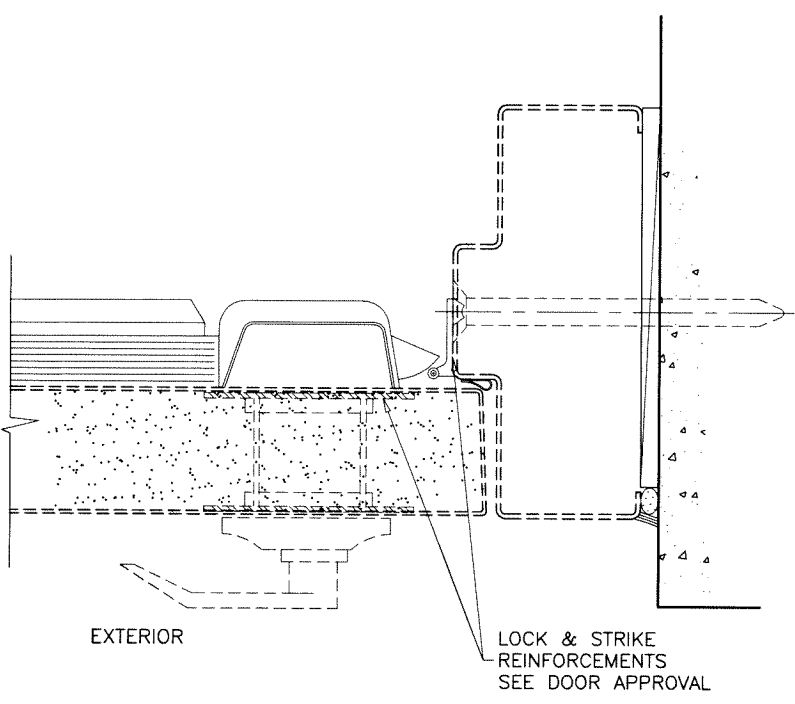
SECTION C-C '6200' SERIES RIM EXIT DEVICE
