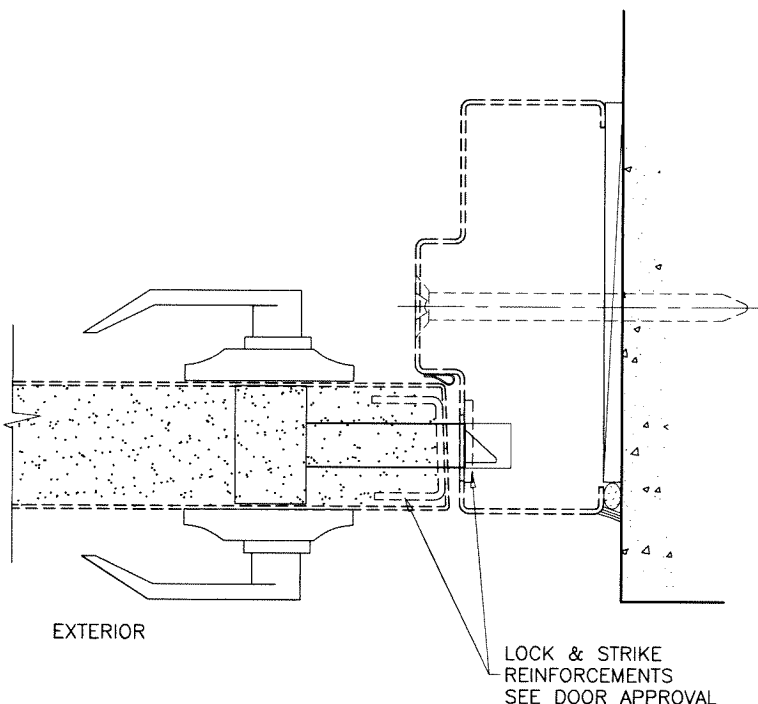
SECTION B-B 'MR' SERIES MORTISE LOCK
