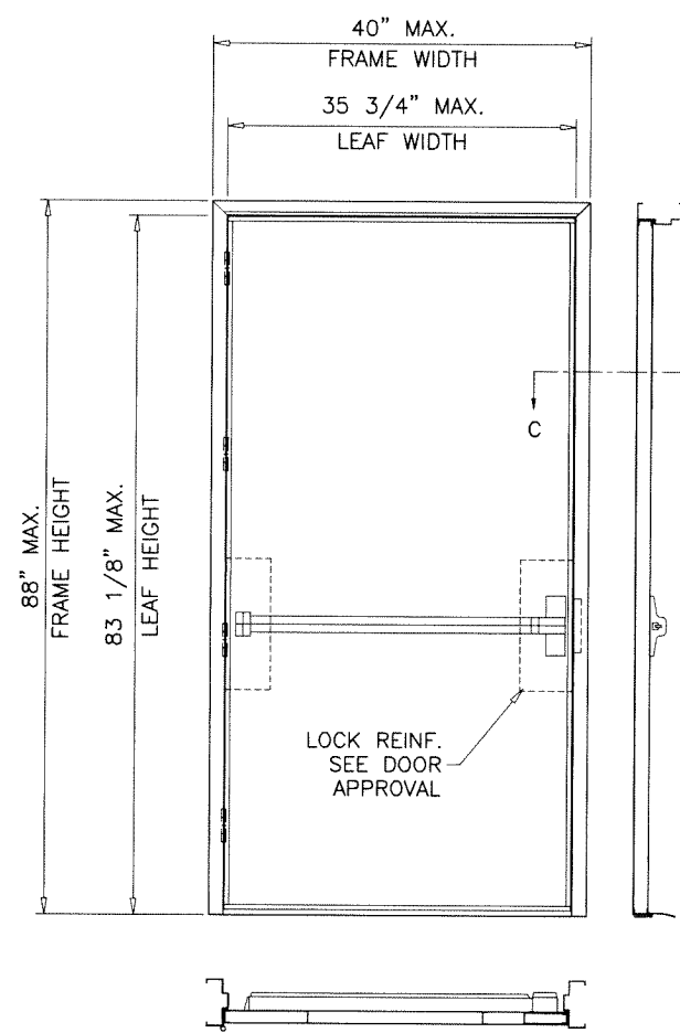
OUTSWING SINGLE STEEL DOOR
